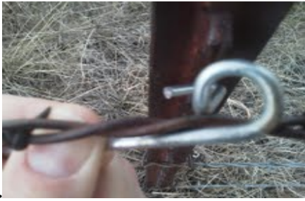
1. Slide wire into loop
